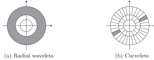
Figure 1.6 Tiling of the frequency domain by radial wavelets and curvelets.
