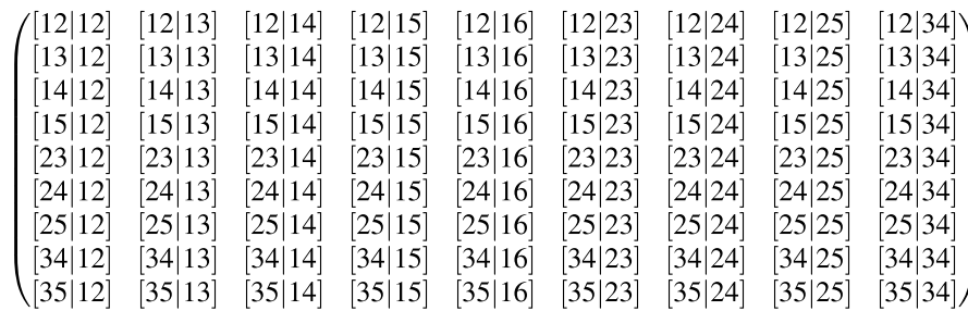
Fig. 3. A matrix representing a determinantal relation.
